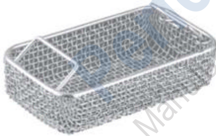
MESH TRAY PS-3522 240x130x50mm PS-3523 240x130x60mm PS-3524 240x250x50mm PS-3525 240x250x60mm PS-3526 480x250x50mm PS-3527 480x250x60mm PS-3528 480x250x70mm
